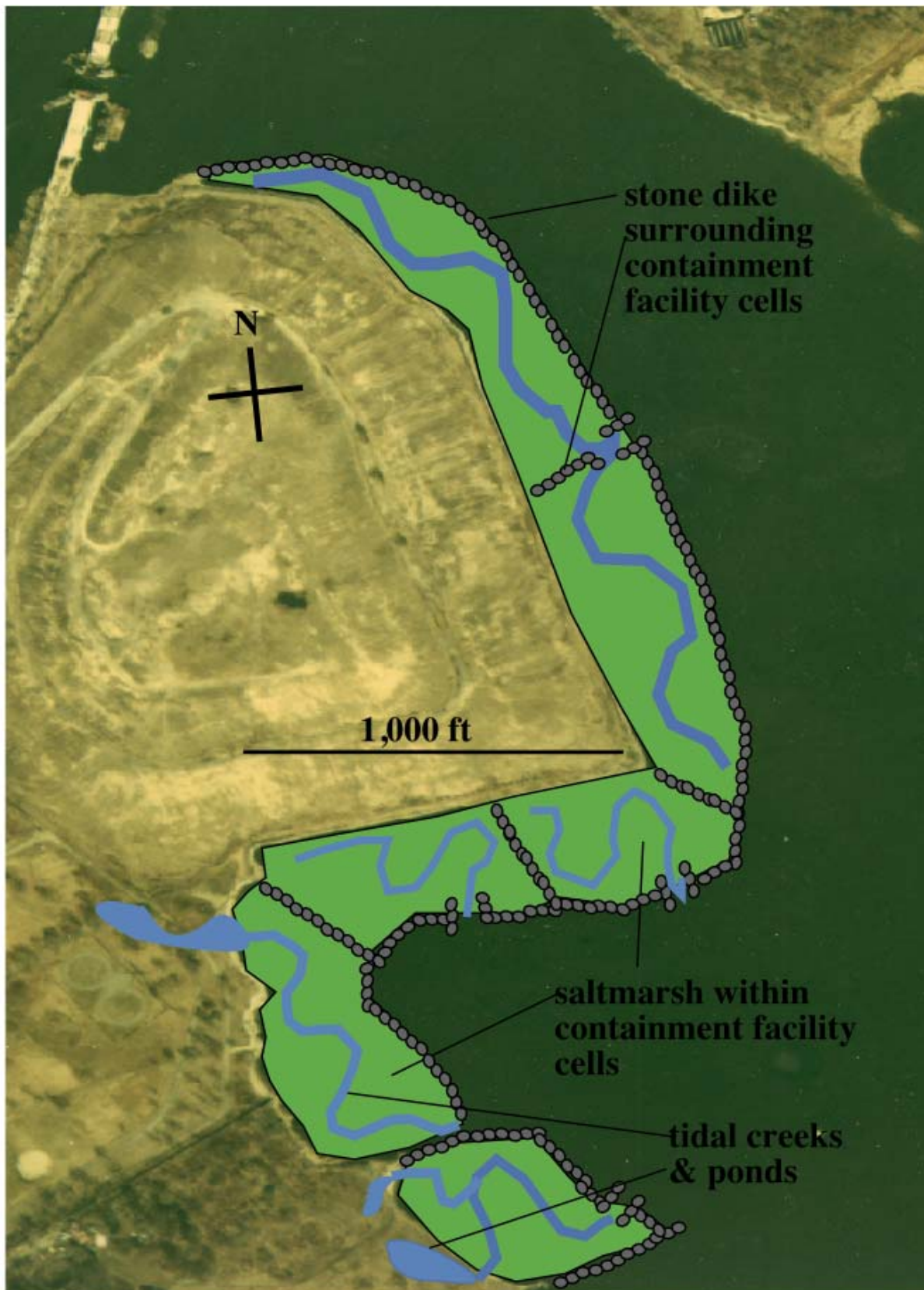
Figure 2. Stone dike confined containment facility, saltmarsh, and tidal creeks. As shown here, approximately 30 acres of saltmarsh could be constructed on dredged sediments surrounding the Pelham Bay Landfill and the southern tier of Pelham Bay Park.
