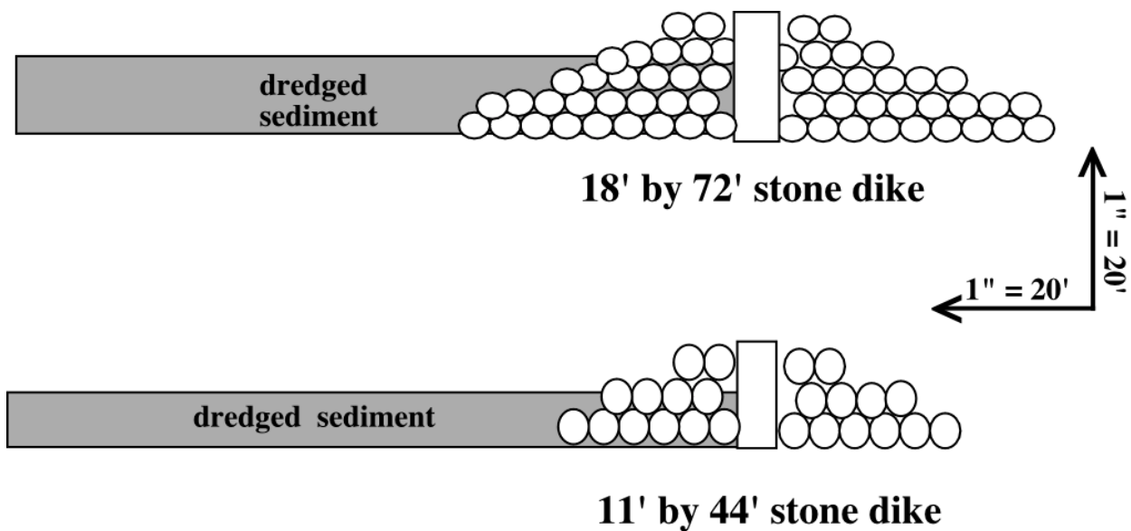
Figure 3. Dimensions of Stone Dike to be Constructed. Height will vary between 11 feet and 18 feet. Sediment will be infilled to between the mid and high tide marks, the preferred growth area of Spartina alterniflora . The total height of the stone dike planned to be three feet above the high tide mark. Hydrodynamic studies will determine the actual height necessary dissipate wave energy at the maximal fetch.
